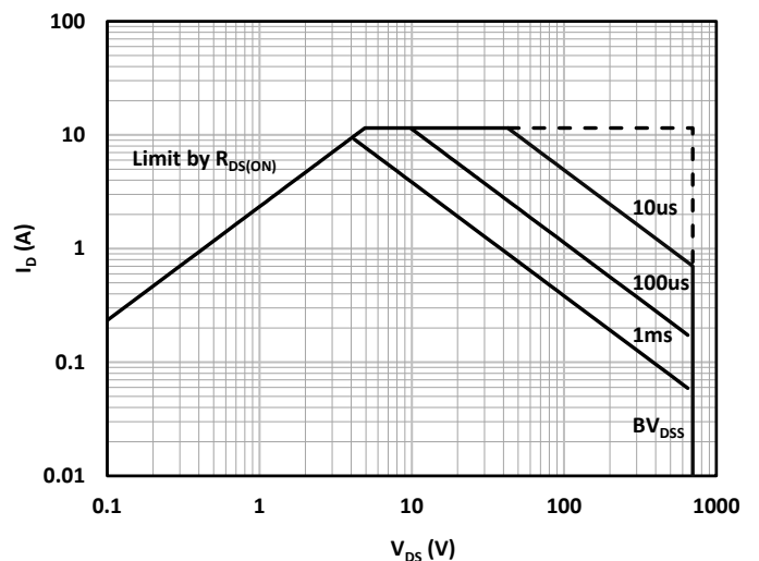
Figure 12. Safe Operating Area, T_J=125^\circ\text{C}
