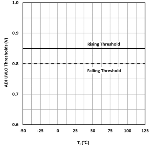
Fig. 8. ADJ UVLO Thresholds vs Temperature
