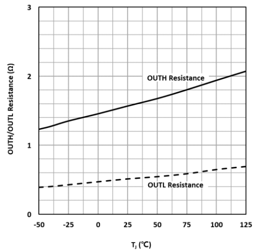
Fig. 12. OUTH/OUTL Resistance vs Temperature
